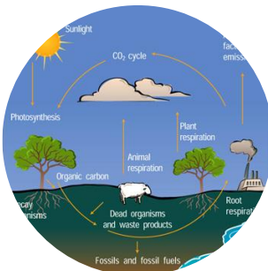
Carbon Cycle
